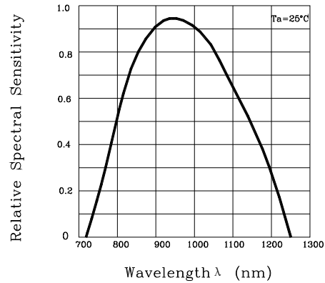
Fig. 2 Spectral Sensitivity
